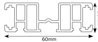
DECKING SIDE
