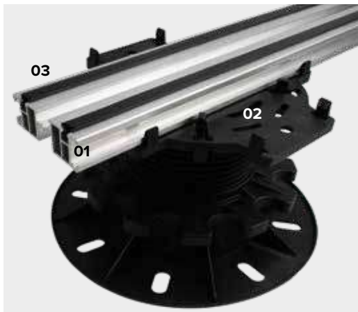
PAVING SIDE
