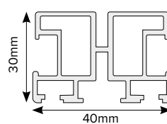
DECKING SIDE
